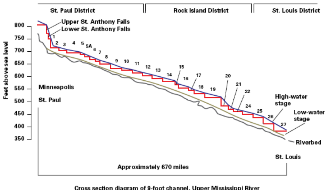
Figure 3. Elevation profile of the Upper Mississippi River System showing the increase in low-flow river stage caused by navigation dams (numbered 1-27). The river at flood stage exceeds stages required for navigation and is allowed to flow freely through and over dams (after Theiling 1999).
