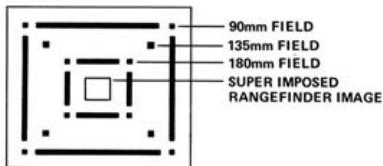
Viewfinder Window
